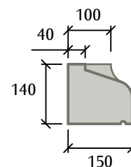
Stooped Cill
