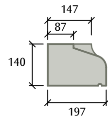
Stooped Cill
