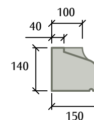
Once Stooped Cill
