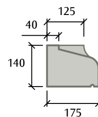
Once Stooled Cill
