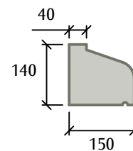
Slip Cill
