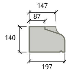
Once Stooped Cill
