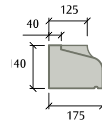
Stooled Cill
