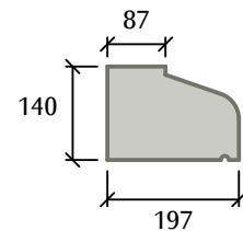
Slip Cill
